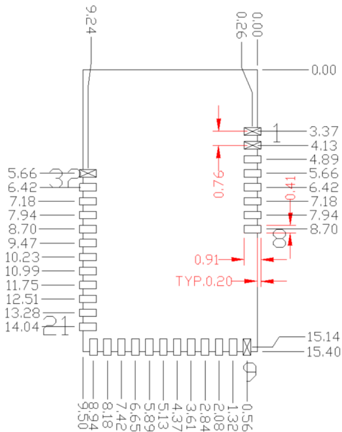
Top View (Seen on Host PCB)
