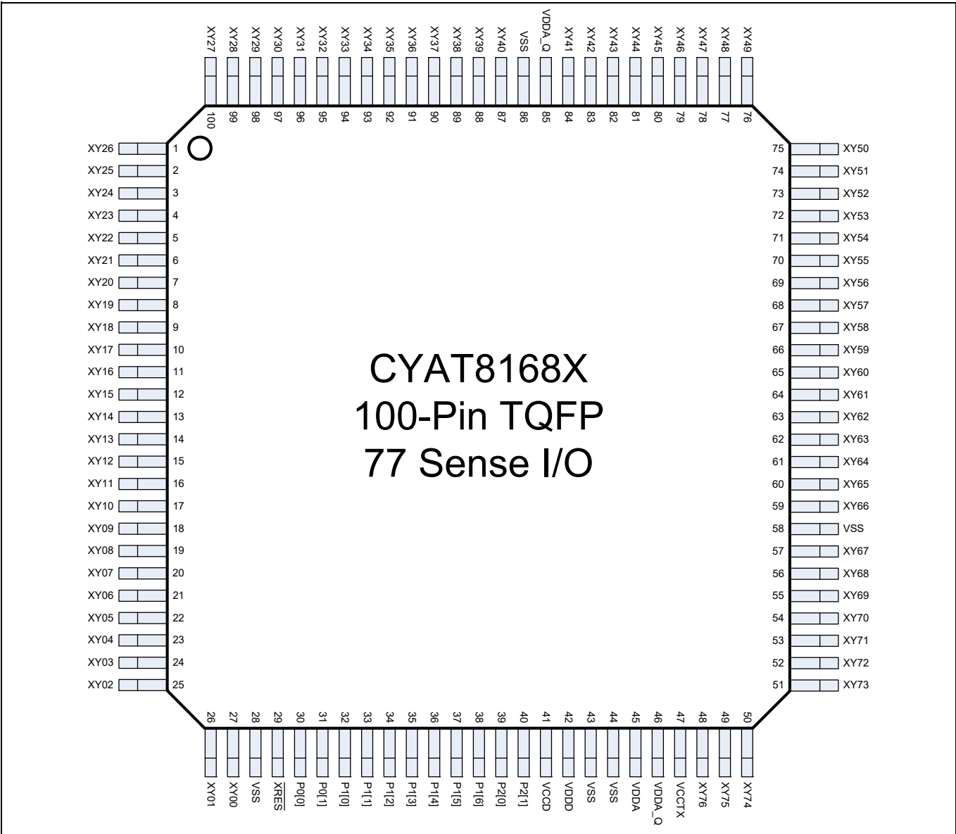
Figure 13 100-pin TQFP, 77 sense I/O CYAT8168X
