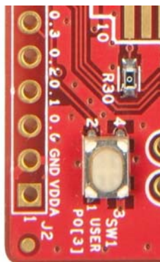
Figure A-9. User Switch on the Board
