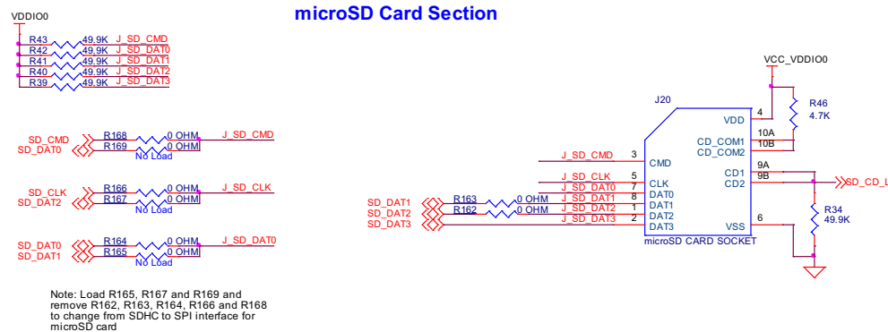
Figure 5-22. microSD Card SPI Multiplexing
