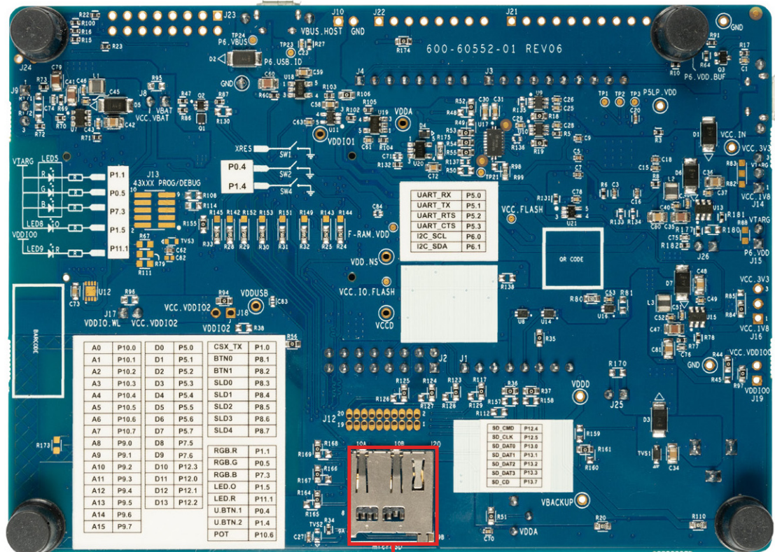
Figure 3-5. PSoC 64 “Secure Boot” Wi-Fi BT Pioneer Board - Bottom View
