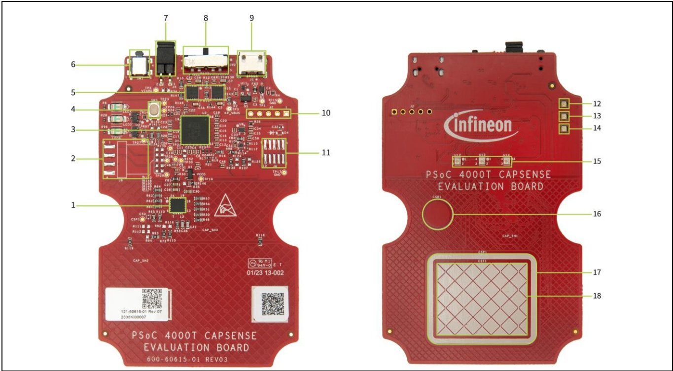
Figure 4 PSoC™ 4000T CAPSENSE™ EVB details
