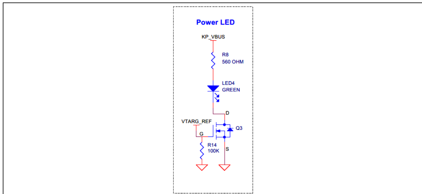
Figure 20 Schematic of power LED indication (LED4)
