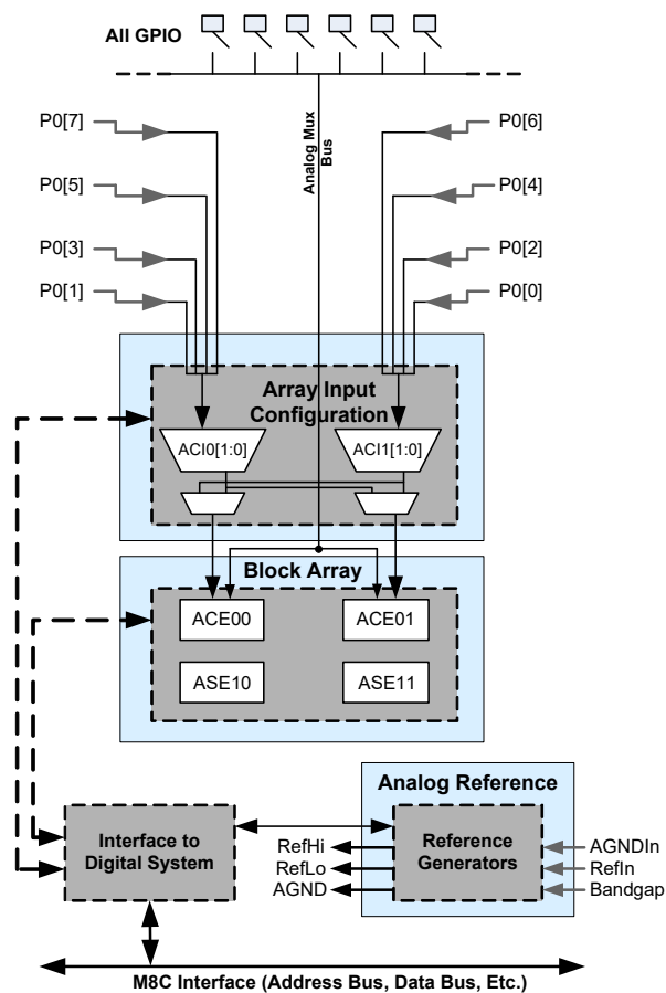
Figure 7. Analog System Block Diagram for CY8C28x13 Devices
