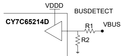
Figure 11. GPIO VBUS Detection, VBUS > VDDD
