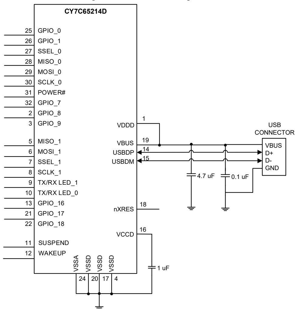
Figure 5. Bus-Powered Configuration
