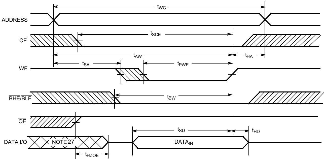
Figure 7. Write Cycle No. 1: \overline{\text{WE}} Controlled [24, 25, 26]
