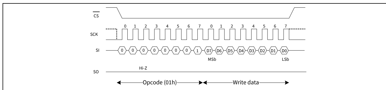
Figure 9 WRSR bus configuration (WREN not shown)
