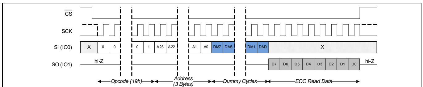
Figure 72 ECC read (ECCRD) in SPI mode
