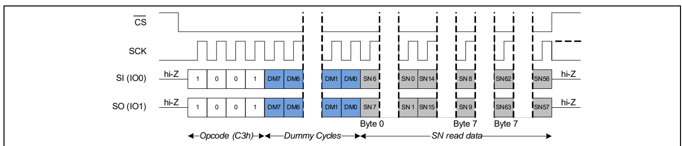
Figure 97 Read serial number (RDSN) in DPI mode
