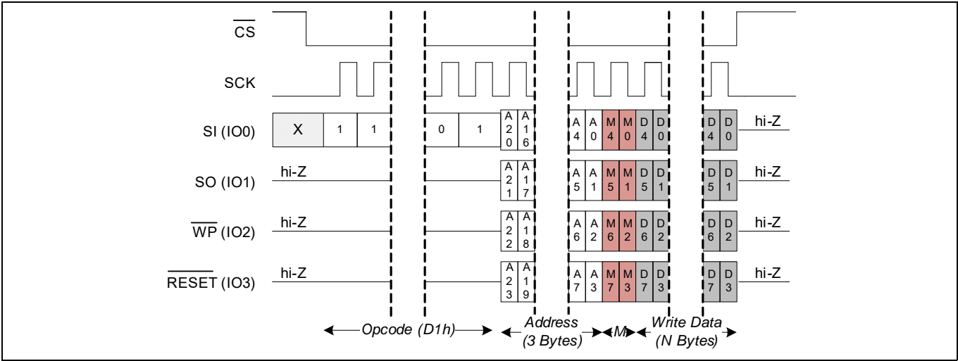
Figure 51 Quad I/O write (QIOW)
