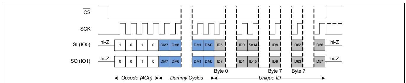
Figure 91 Read unique ID in DPI mode
