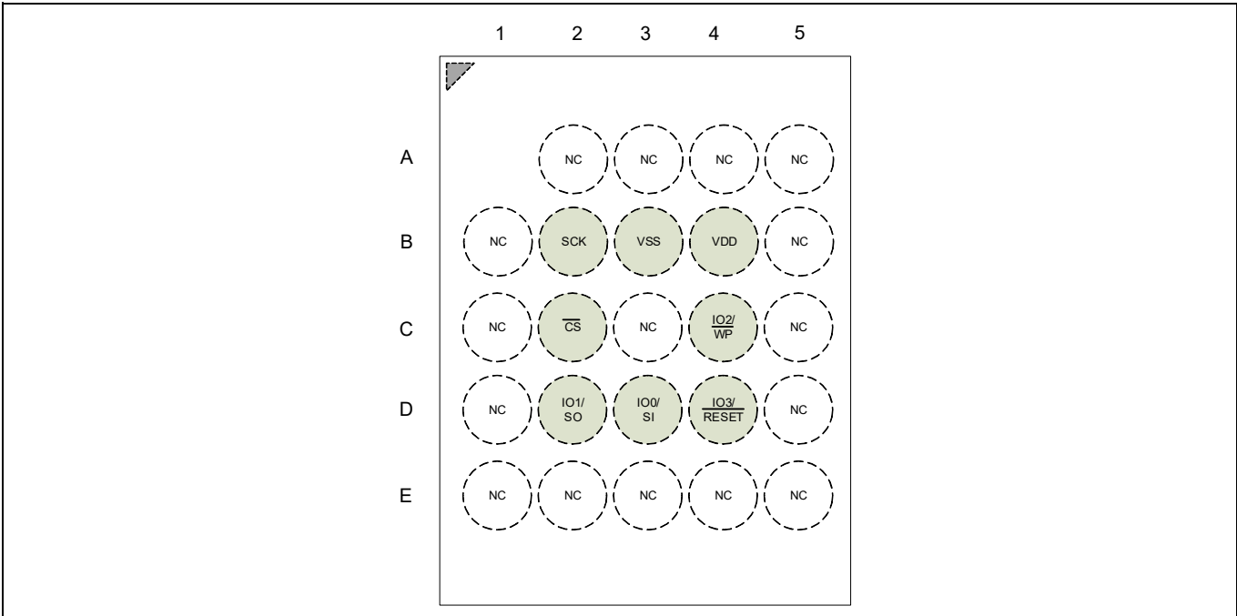
Figure 1 24-ball BGA pinout
