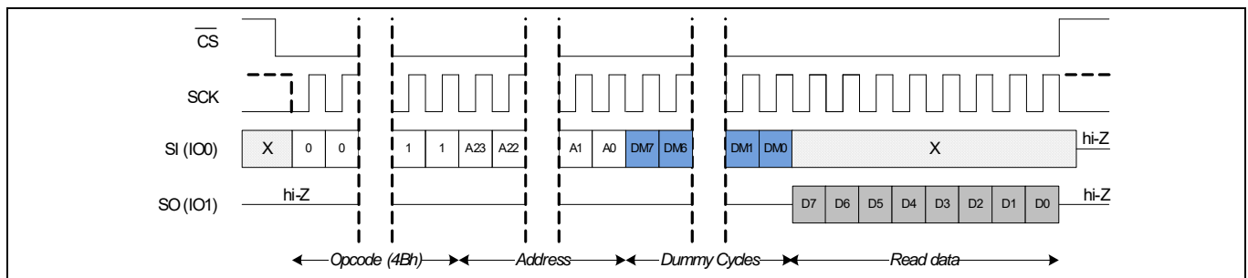
Figure 69 Special sector read (SSRD) in SPI mode
