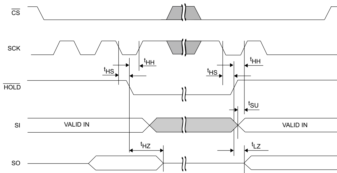
Figure 17. \overline{\text{HOLD}} Timing
