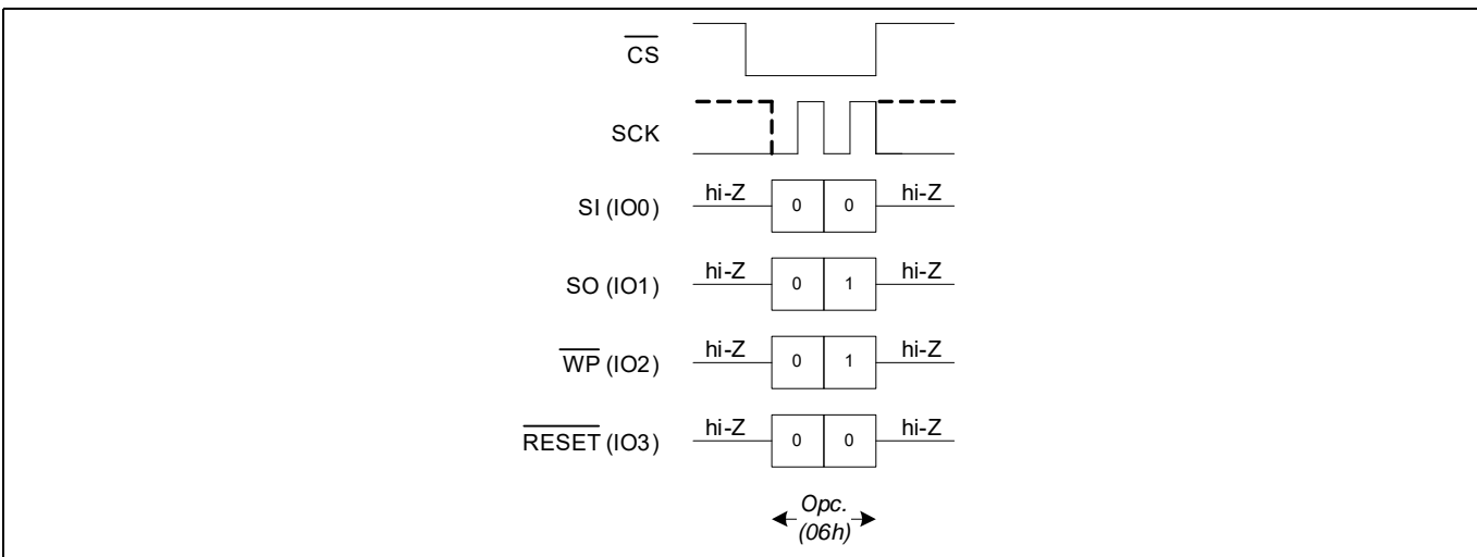
Figure 8 WREN bus configuration in QPI mode
