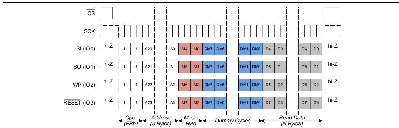
Figure 63 Quad I/O read (QIOR) in QPI mode
