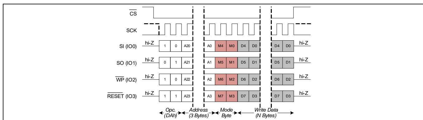
Figure 45 Fast write (FAST_WRITE) in QPI mode
