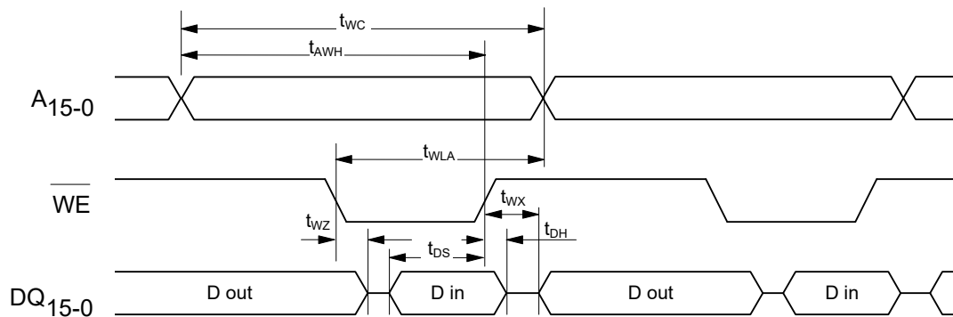
Figure 10. Write Cycle Timing No. 3 ( \overline{CE} LOW) [8]
