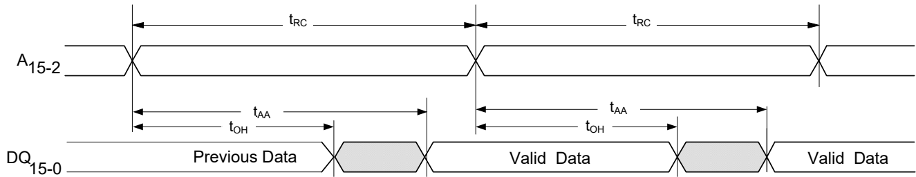
Figure 6. Read Cycle Timing No. 2 ( \overline{\text{CE}} Controlled)
