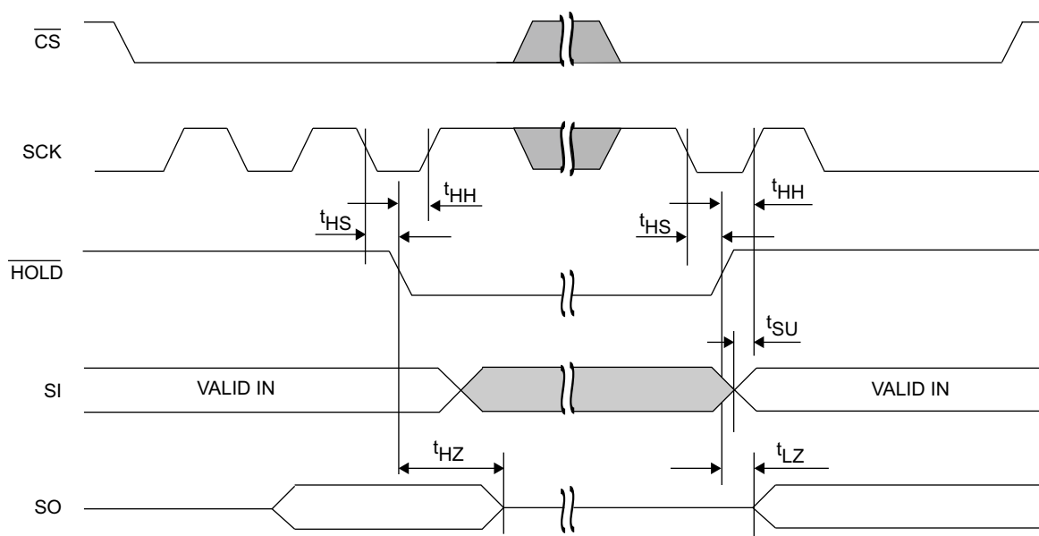
Figure 14. \overline{\text{HOLD}} Timing
