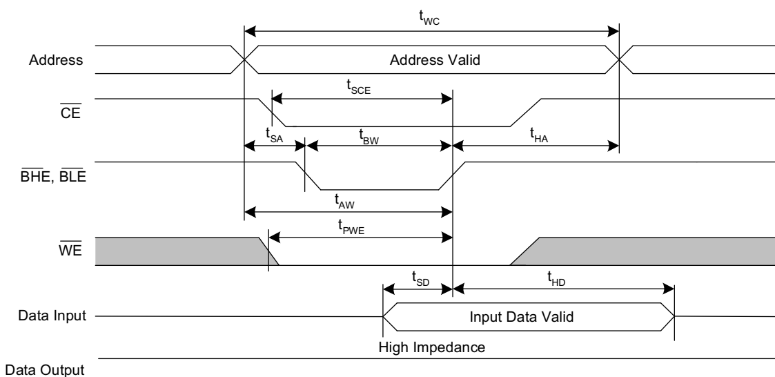
Figure 9. SRAM Write Cycle No. 3 ( \overline{\text{BHE}} and \overline{\text{BLE}} Controlled) [24, 25, 26]
