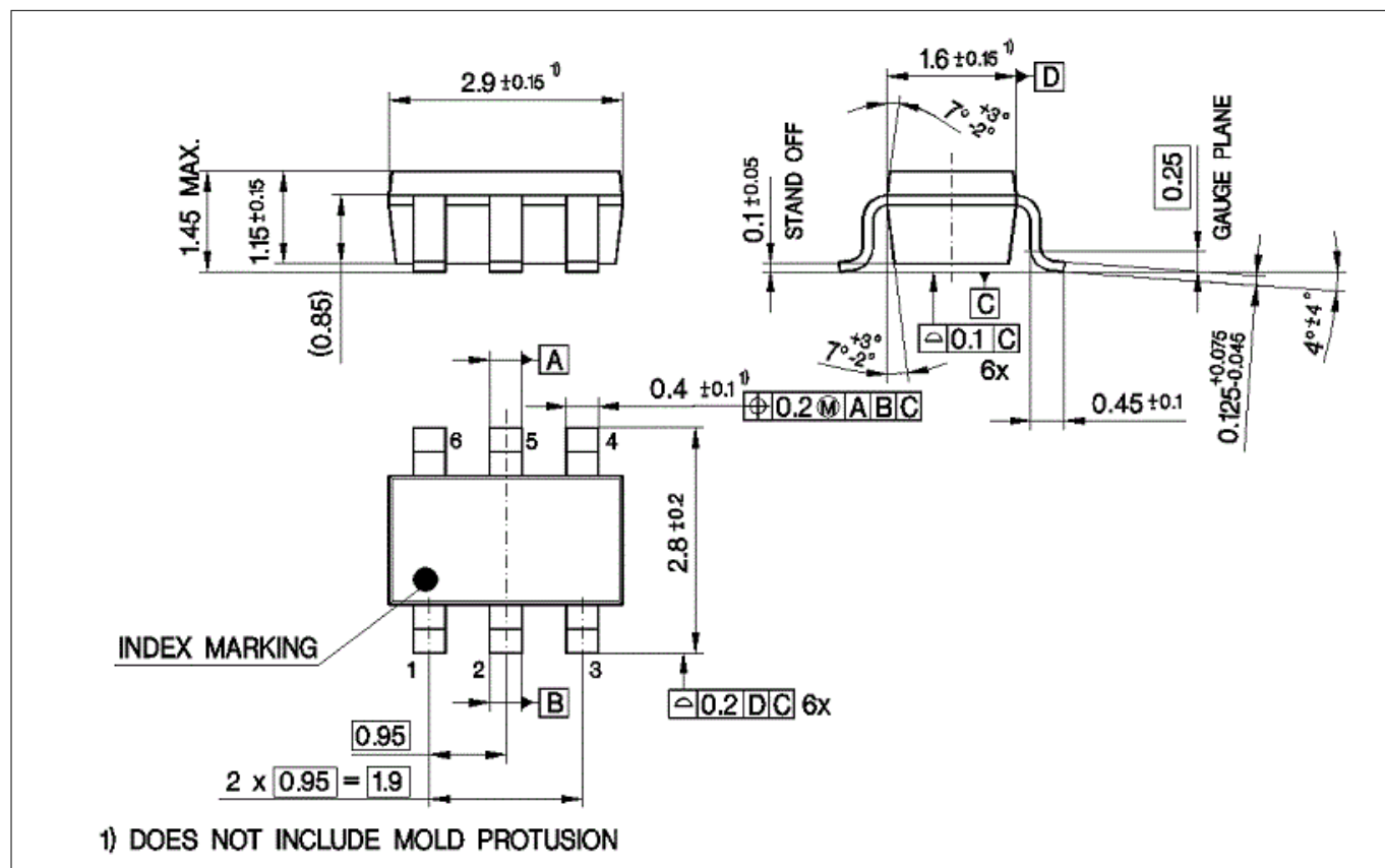
Figure 9 Package Drawings
