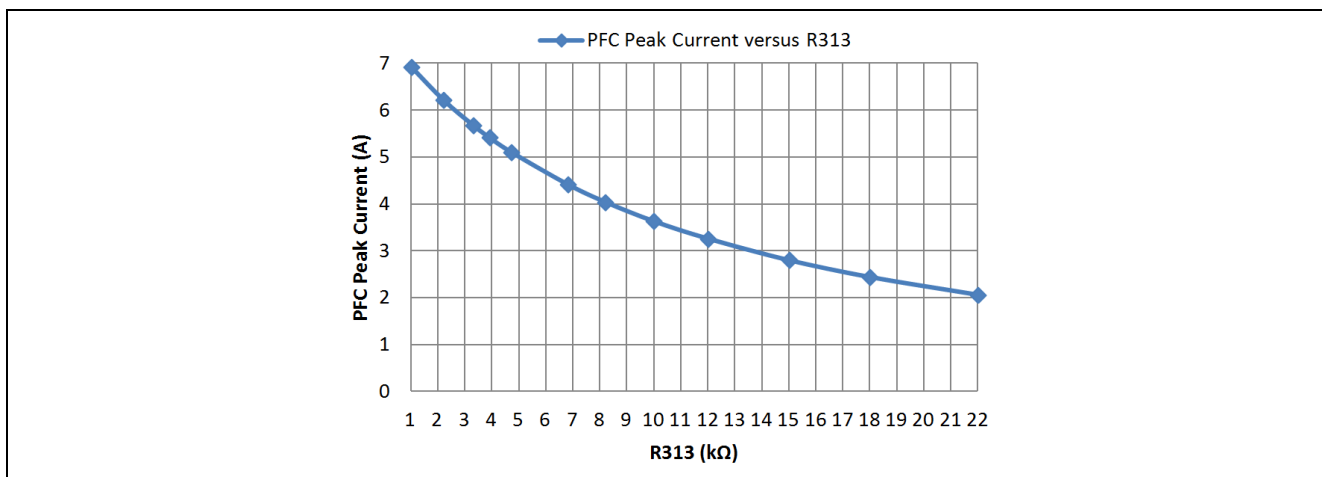
Figure 9 PFC Peak Current versus R313
