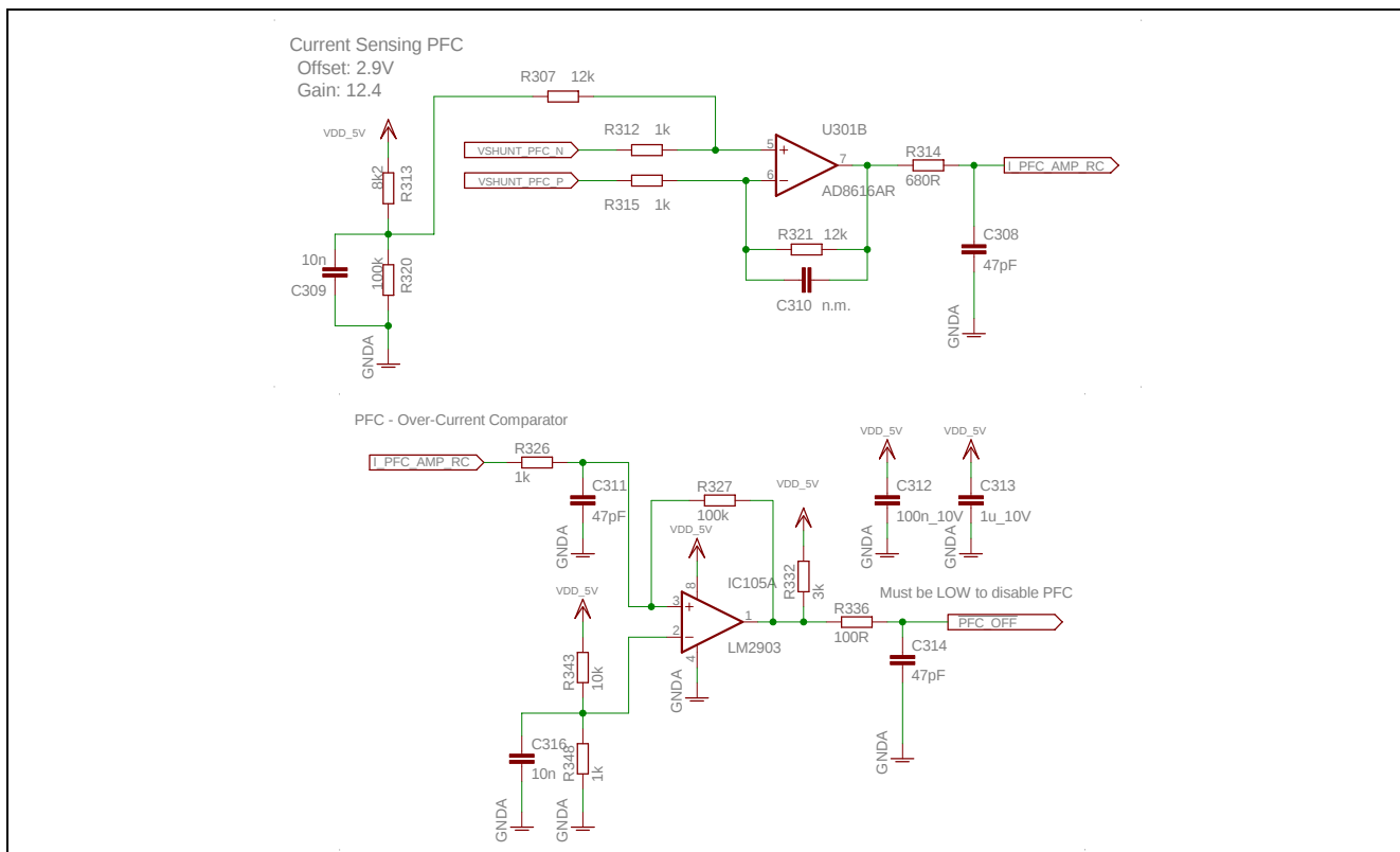
Figure 8 PFC Current Sense and Over Current Protection
