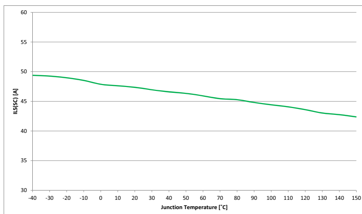
Figure 43 Overload Condition in the Low Voltage Area I_{L5(SC)} = f(T_J; V_S)
