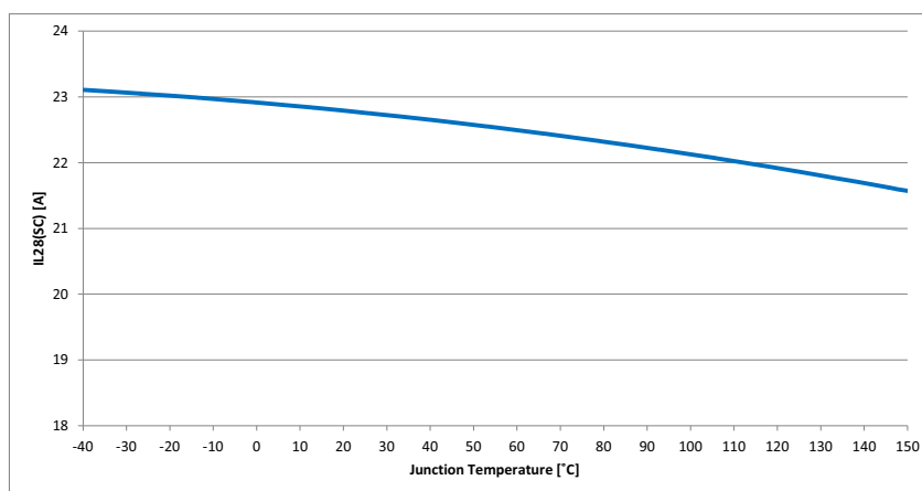
Figure 44 Overload Condition in the High Voltage Area I_{L28(SC)} = f(T_J; V_S)
