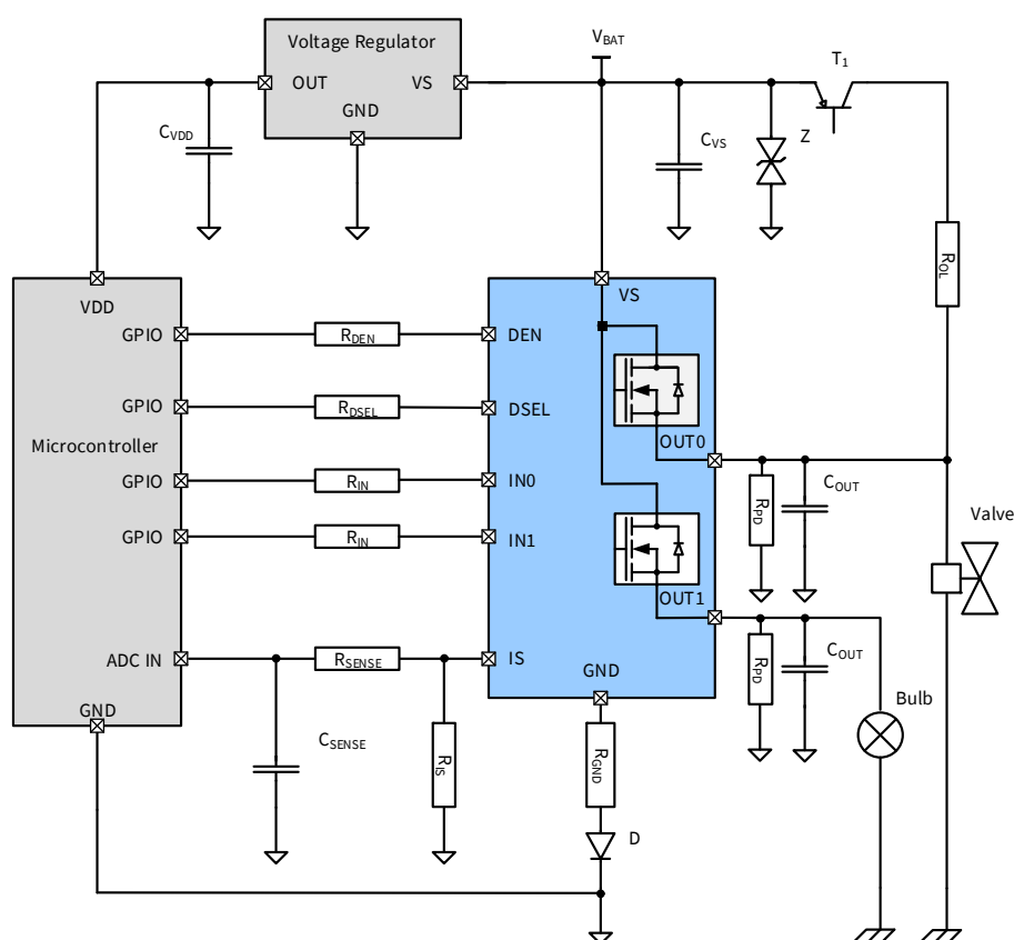
Application Diagram with BTT6030-2ERB
