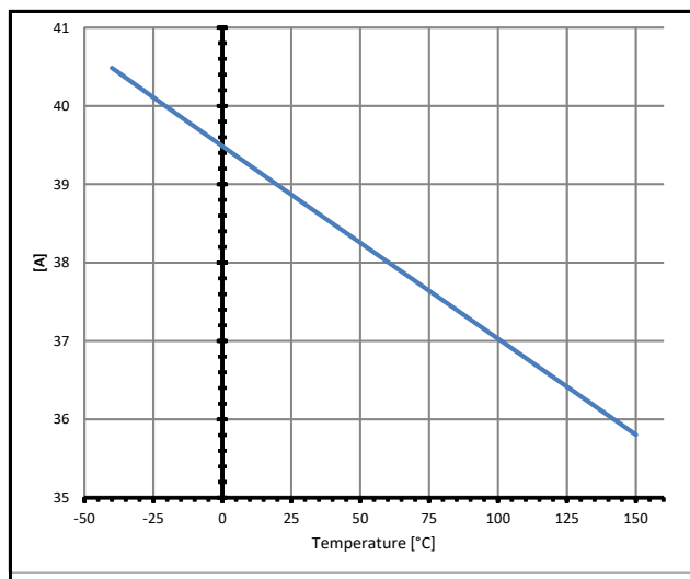
Overload Condition in the High Voltage Area I_{L28(SC)} = f(T_J; V_S)
