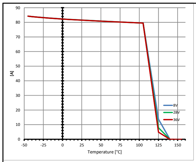
Overload Condition in the Low Voltage Area I_{L5(SC)} = f(T_J; V_S)
