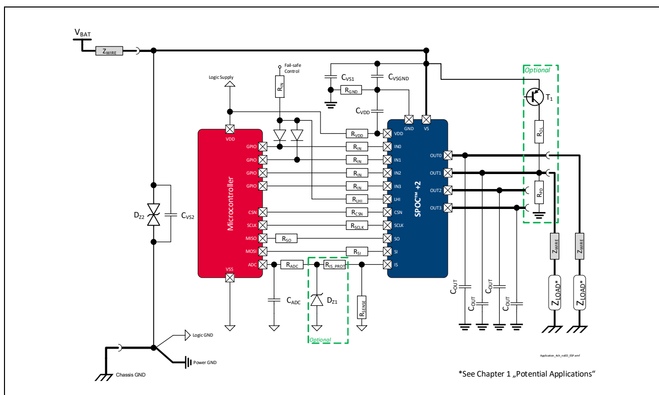
Figure 46 Application Diagram
