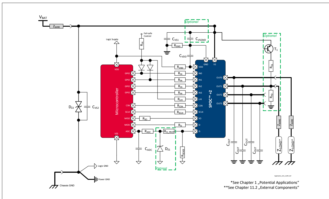
Figure 46 Application Diagram
