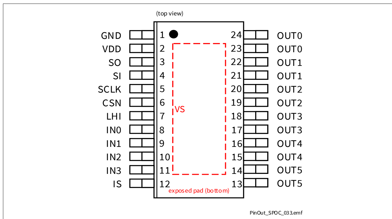
Figure 4 Pin Configuration
