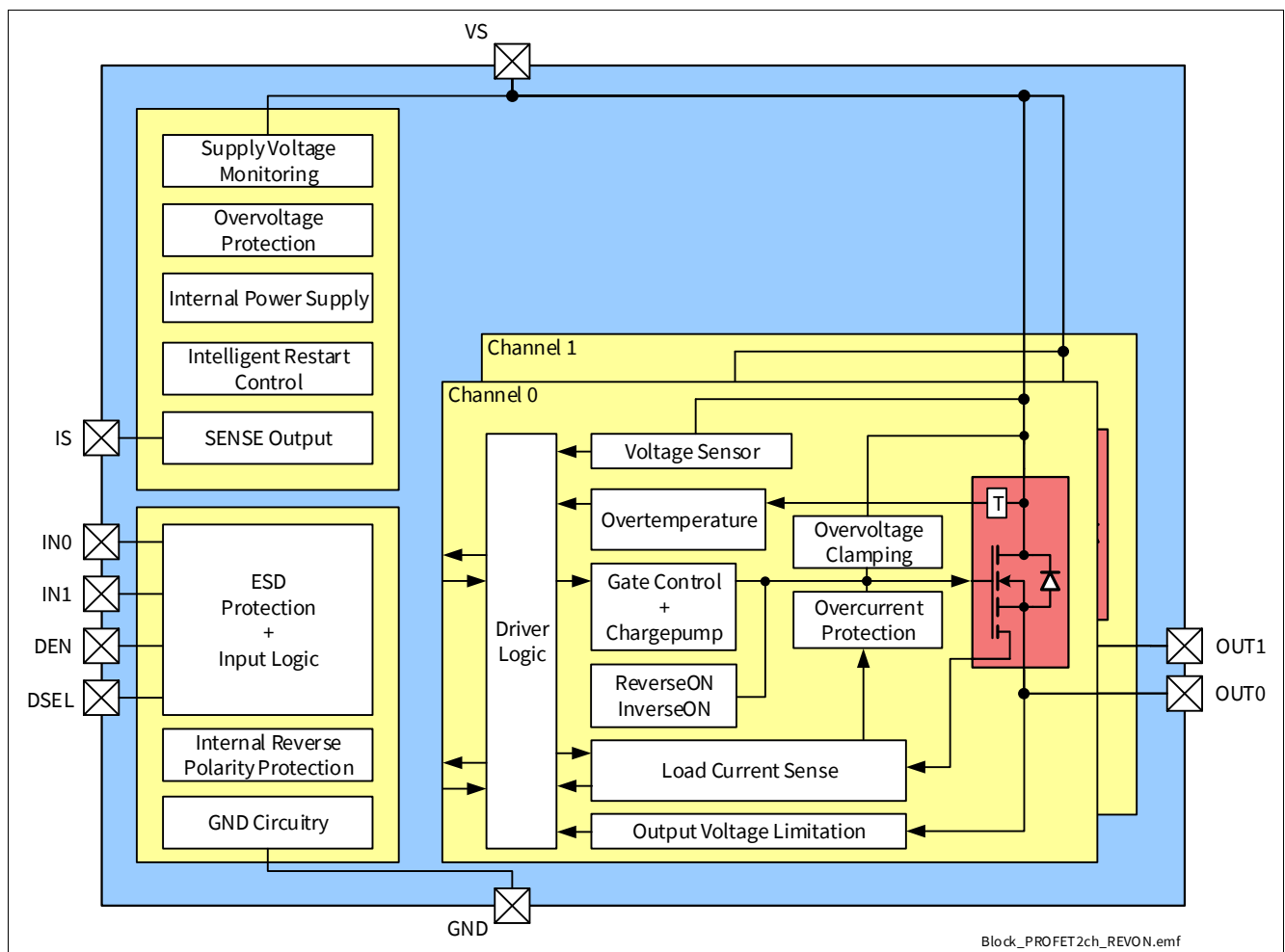
Figure 2 Block Diagram of BTS7040-2EPG
