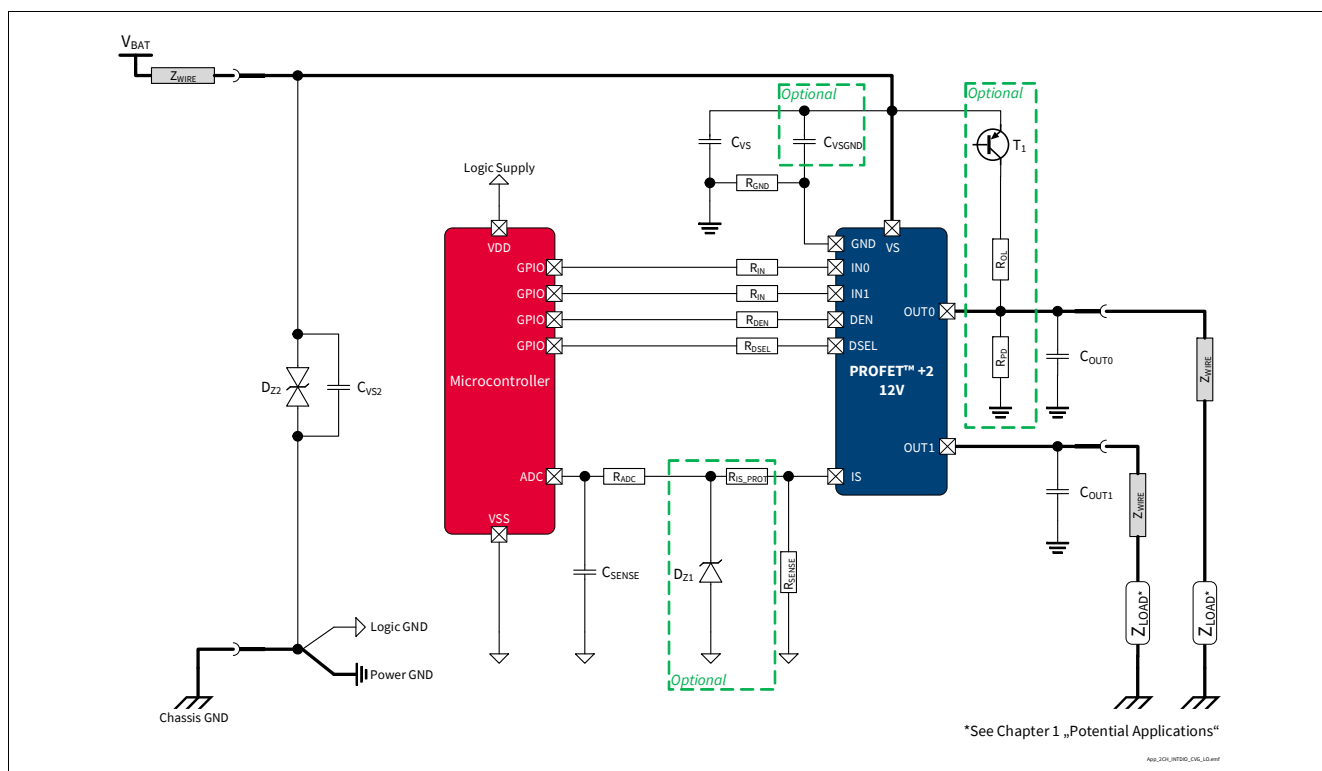
Figure 1 BTS7040-2EPG Application Diagram. Further information in Chapter 10
