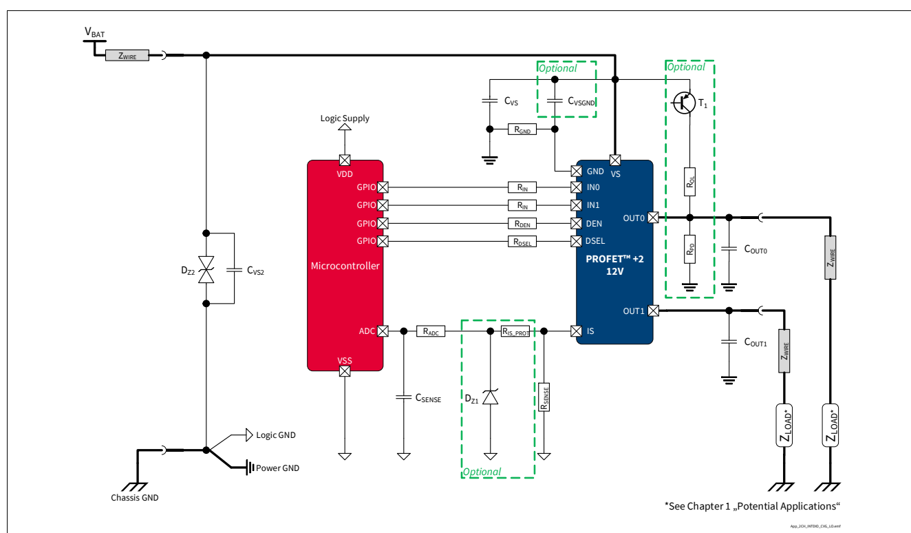
Figure 1 BTS7012-2EPA Application Diagram. Further information in Chapter 10
