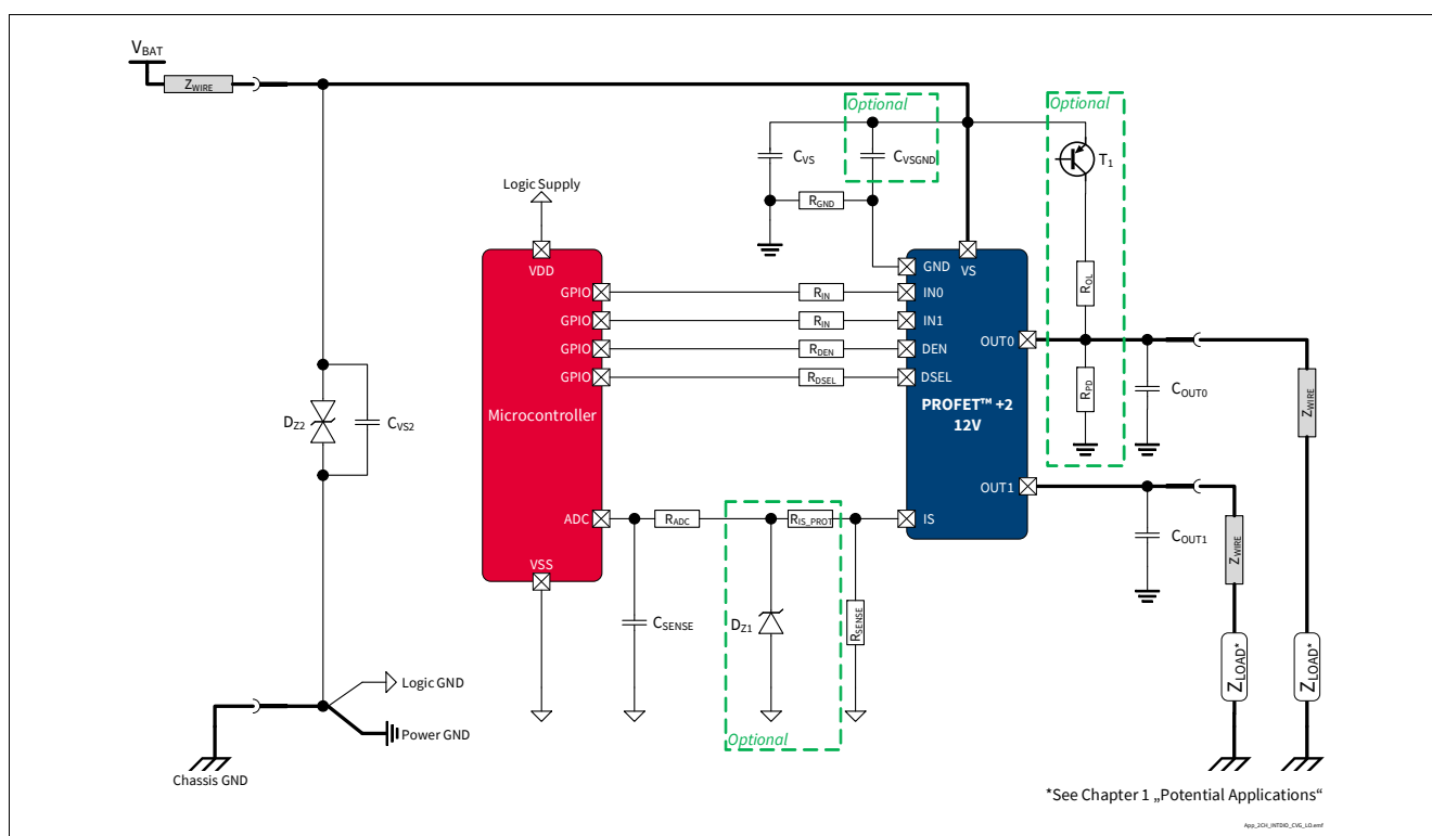
Figure 1 BTS7008-2EPZ Application Diagram. Further information in Chapter 10
