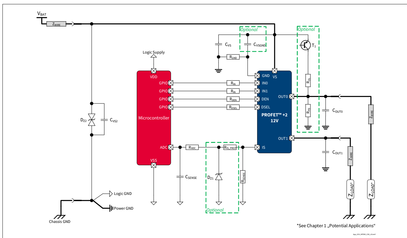
Figure 1 BTS7008-2EPA Application Diagram. Further information in Chapter 10
