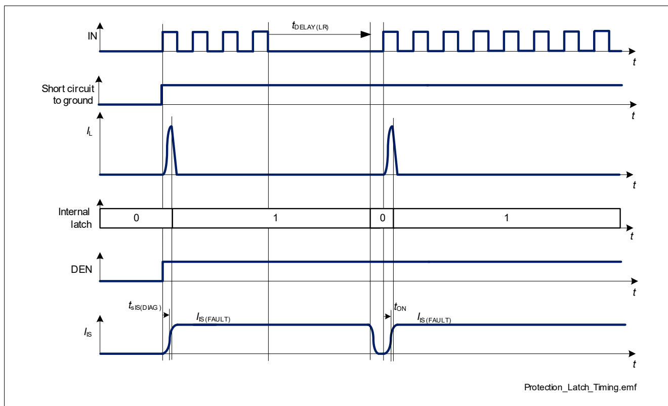
Figure 28 Intelligent Latch Timing Diagram
