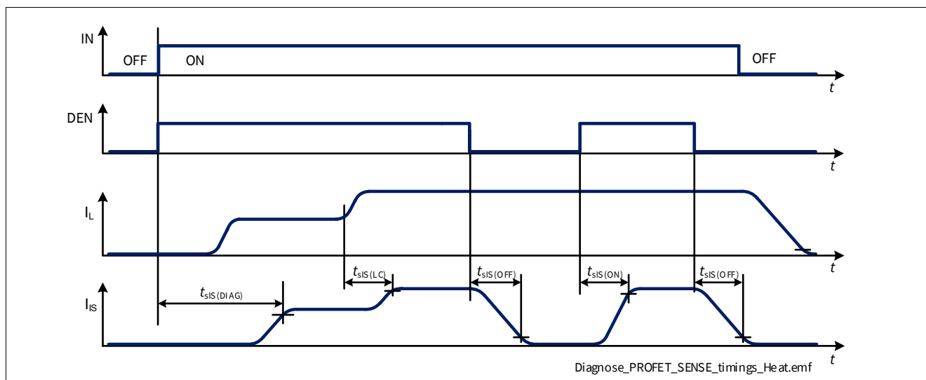
Figure 38 SENSE Settling / Disabling Timing
