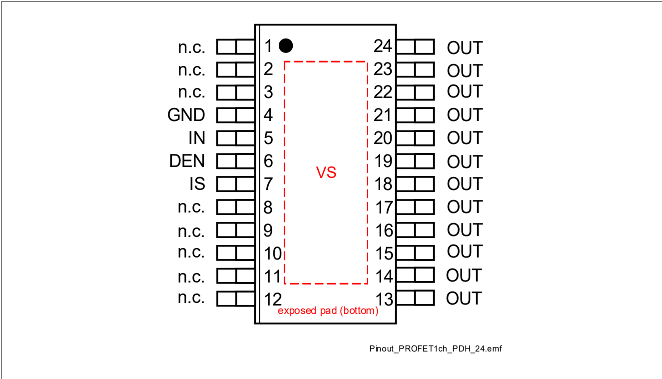
Figure 4 Pin Configuration
