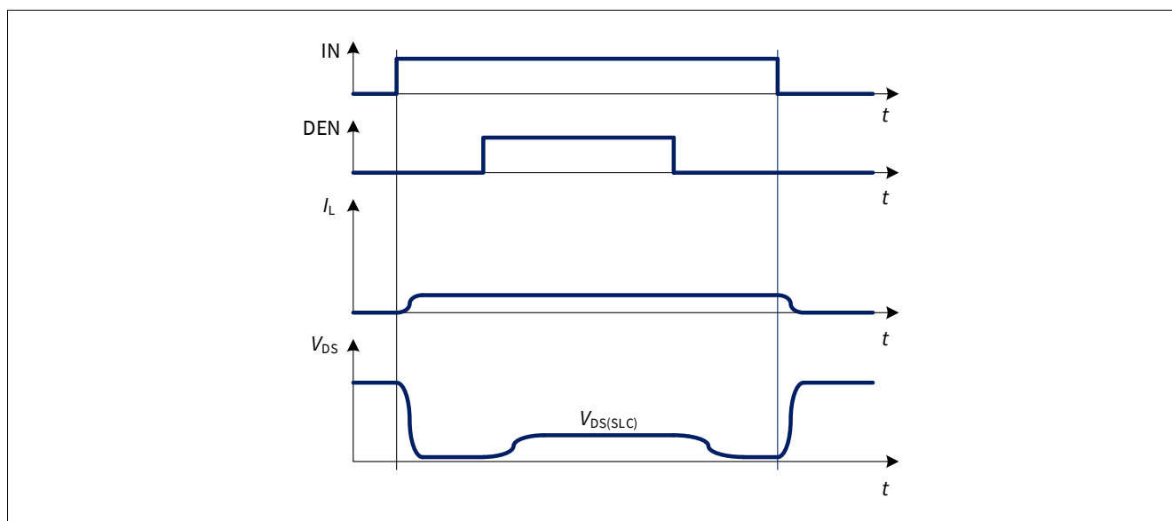
Figure 19 Output Voltage Limitation activation during diagnosis
