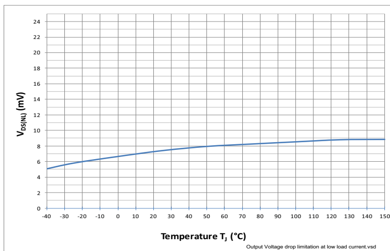
Figure 33 Output Voltage Drop Limitation at Low Load Current V_{DS(NL)} = f(T_J) and V_{DS(NL)} = f(V_S)
