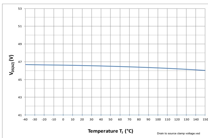
Figure 34 Drain to Source Clamp Voltage V_{DS(AZ)} = f(T_J)
