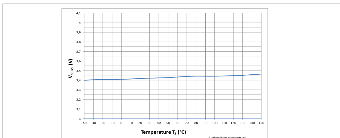
Figure 30 Undervoltage Threshold V_{S(UV)} = f(T_J)
