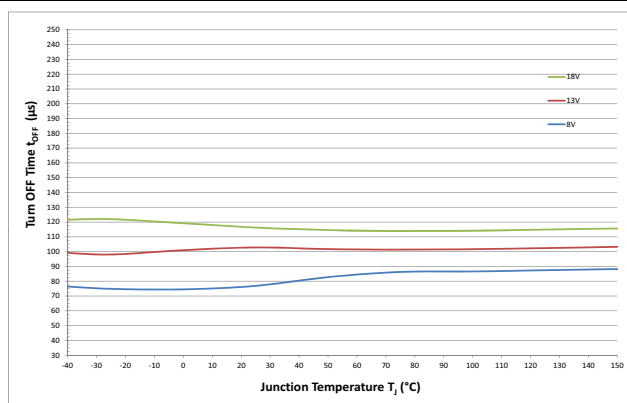
Figure 38 Turn OFF t_{OFF} = f(T_J; V_S) , R_L = 2 \Omega
