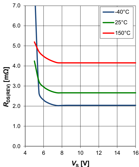
Resistance in ReverSave™ R_{DS(REV)} = f(V_S, T_J), I_L = -15\text{ A}
