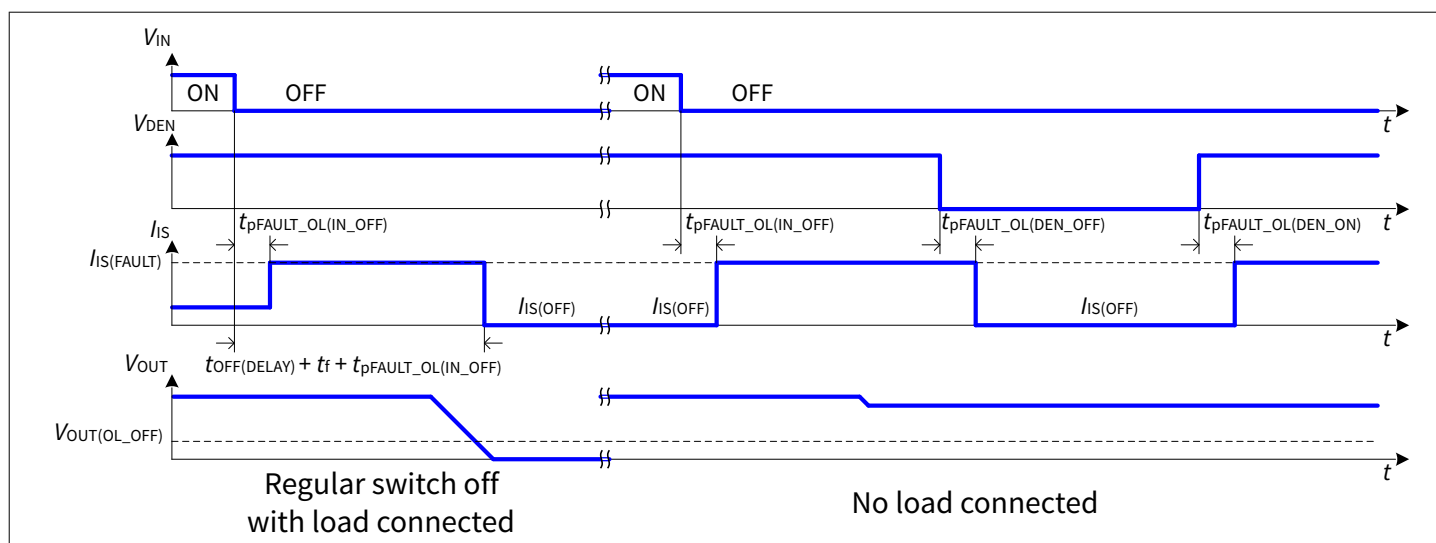
Figure 26 Behavior of the open load detection in off feature with and without load connected
