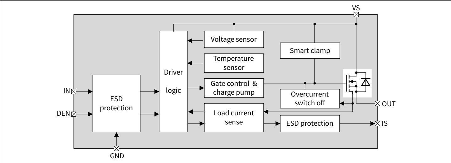
Figure 2 Block diagram
