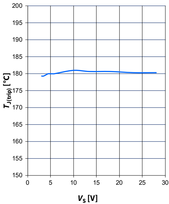
Thermal shutdown temperature T_{J(TRIP)} = f(V_S)
