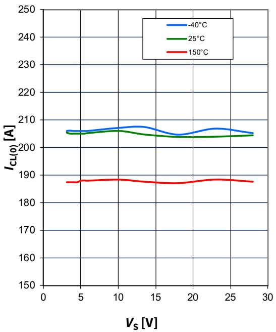
Current trip detection level I_{CL(0)} = f(V_S, T_J)
