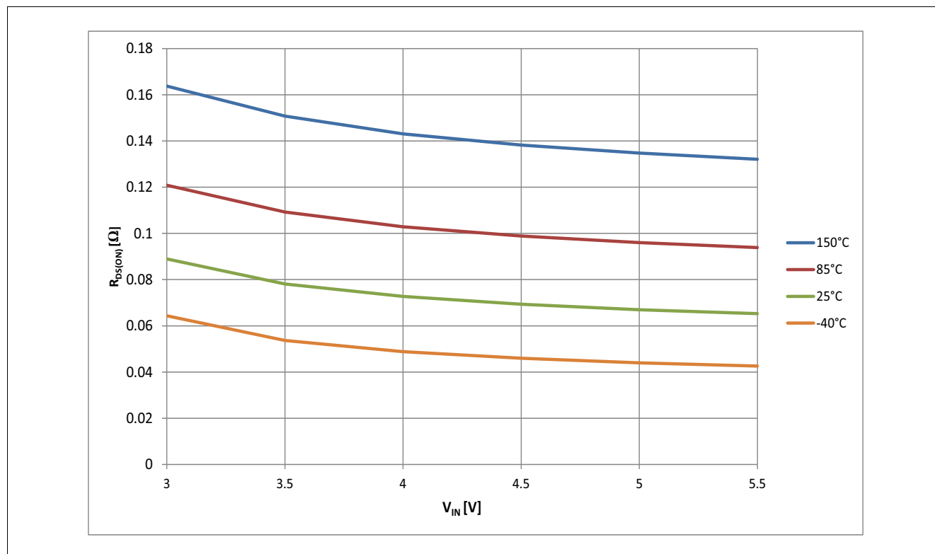
Figure 17 Typical R_{DS(ON)} vs. V_{IN} @ T_j = -40 \dots 150^\circ\text{C} , I_L = I_{L(NOM)}
