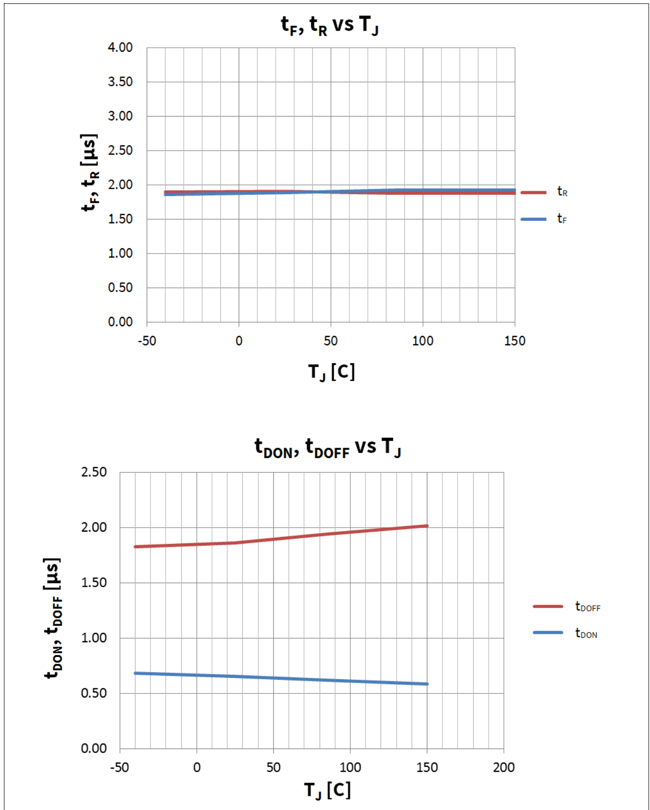
Figure 37 t_F, t_R, t_{DON}, t_{DOFF} vs. T_J = -40; 25; 150^{\circ}C @ R_{SRP} = 5.8k\Omega ; V_{IN} = V_{ENABLE} = V_{DD} = 5V ; V_{BAT} = 13.5V ; R_L = 4.7\Omega
