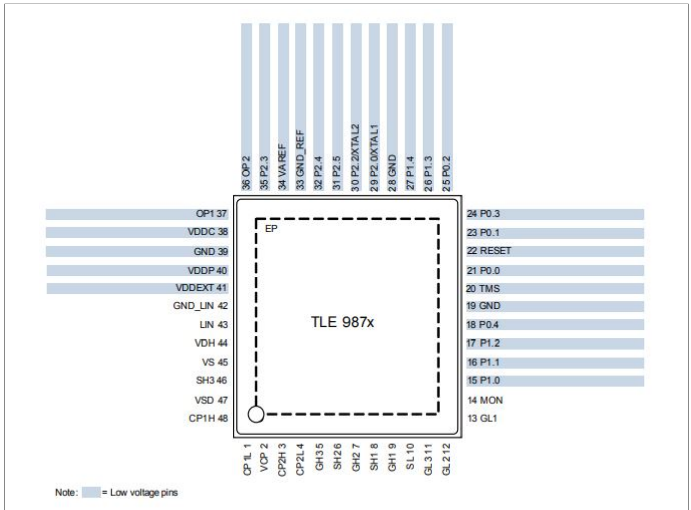
Figure 11 Device pinout TLE9879QXA40
