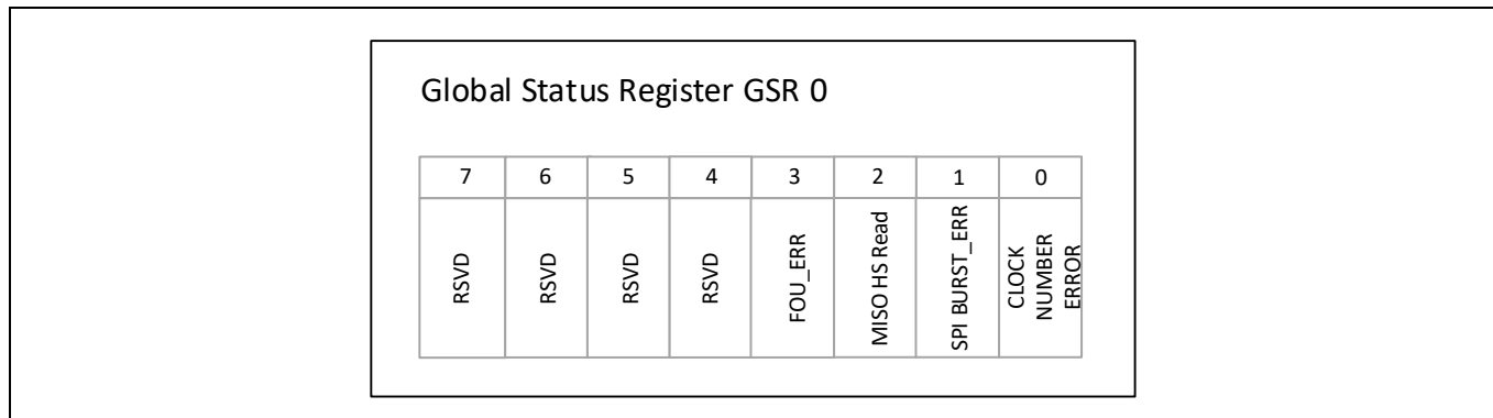
Figure 10 GSR0 Register
