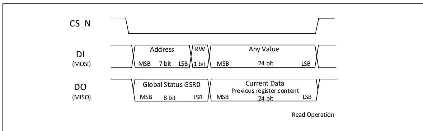
Figure 22 SPI timing read mode
