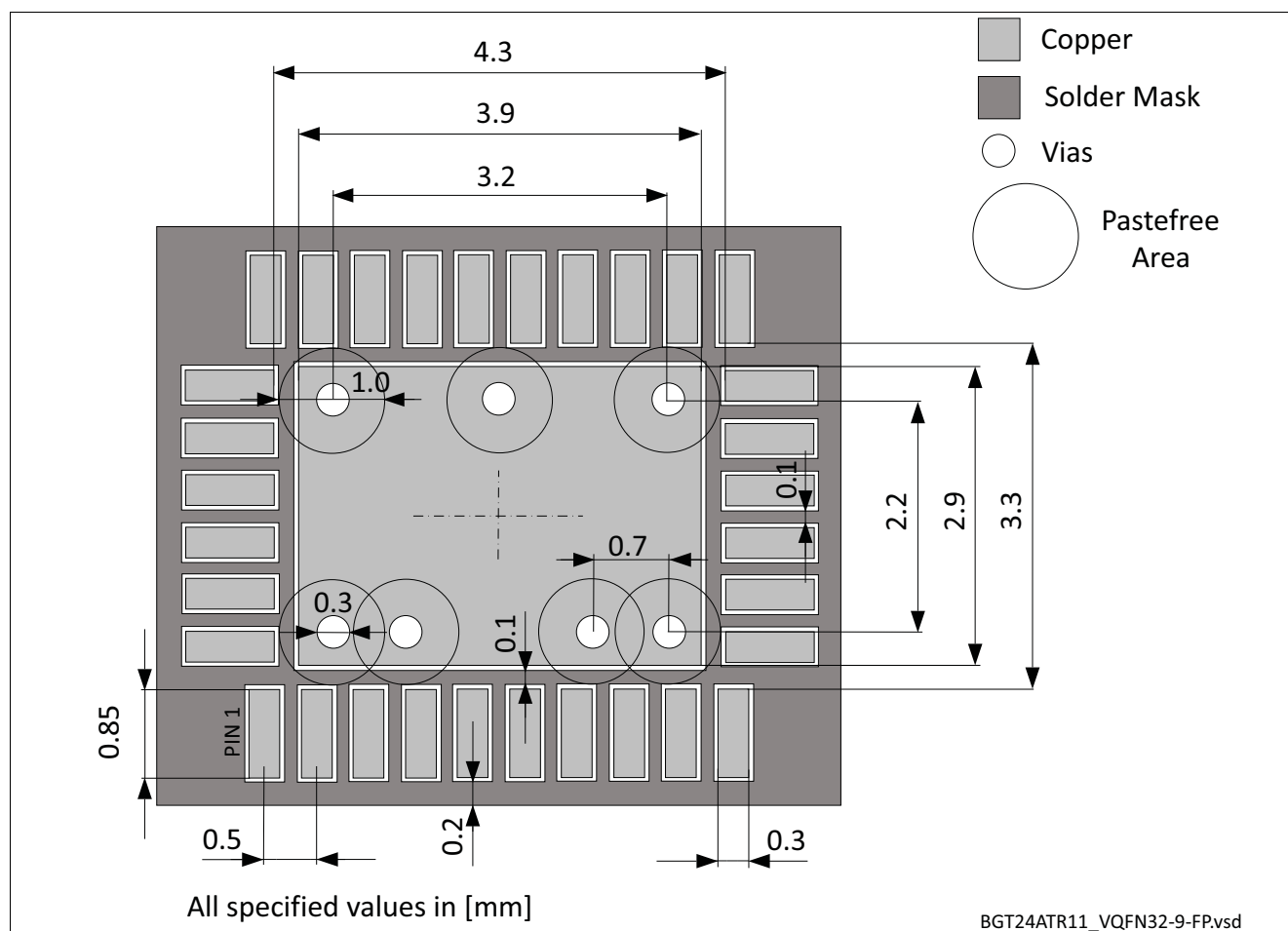
Figure 9 Recommended Footprint and Stencil Layout for the VQFN32-9 Package
