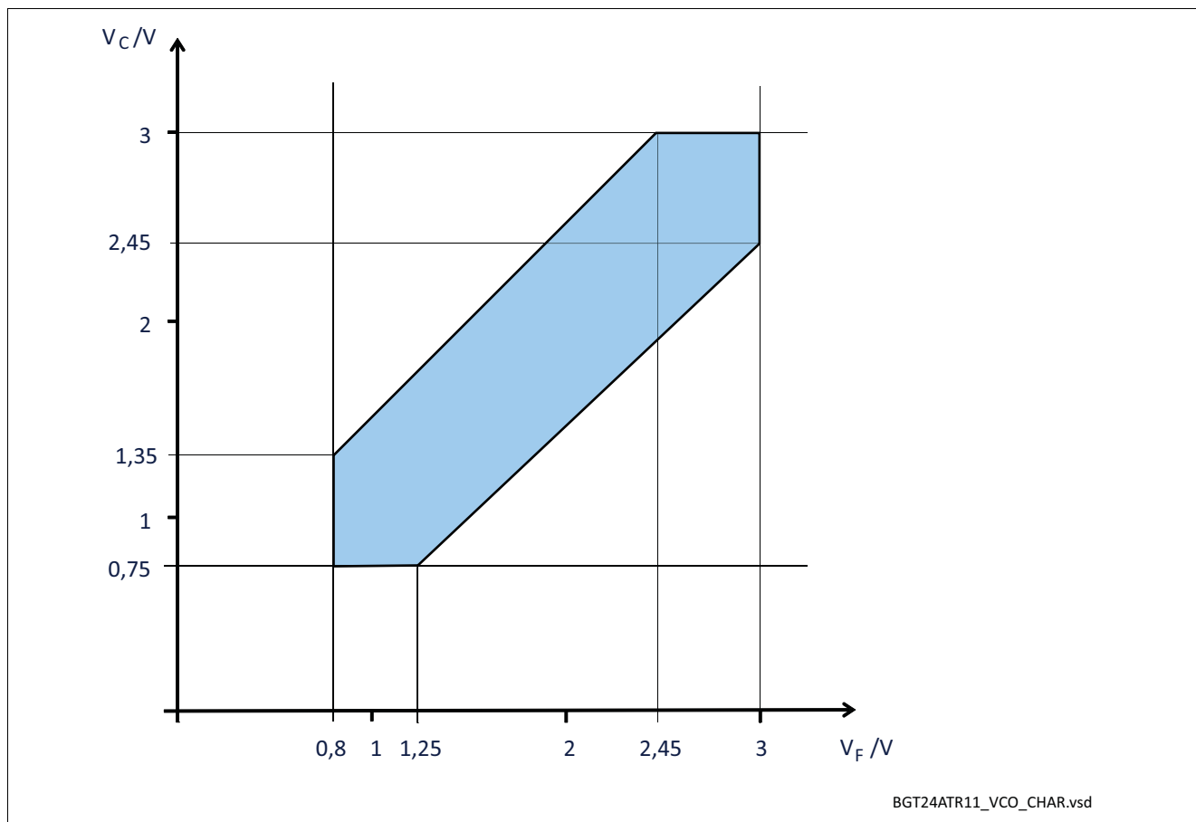
Figure 2 VCO Tuning Window
