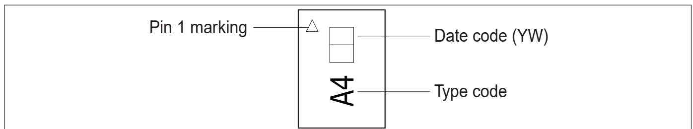
Figure 8: Marking Specification (top view): Date code digits Y and W defined in Table 21/22
