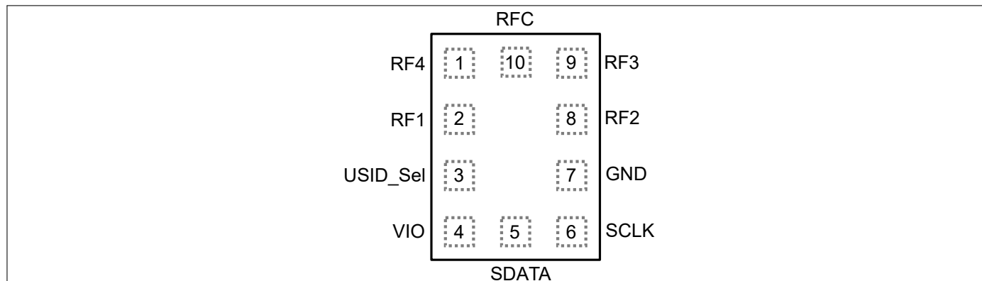
Figure 10: BGSA143ML10 Pin configuration (top view)
