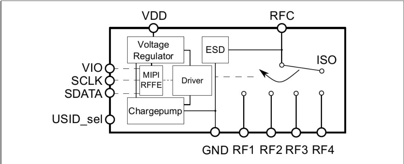
Figure 1 BGS142M2N12 Block diagram
