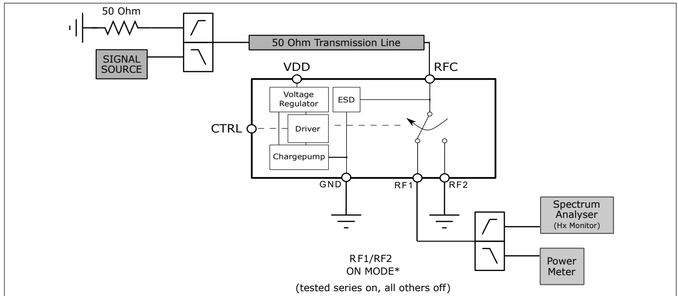
Figure 1: RF operating and Harmonics generation measurement configuration - RFx ON mode
