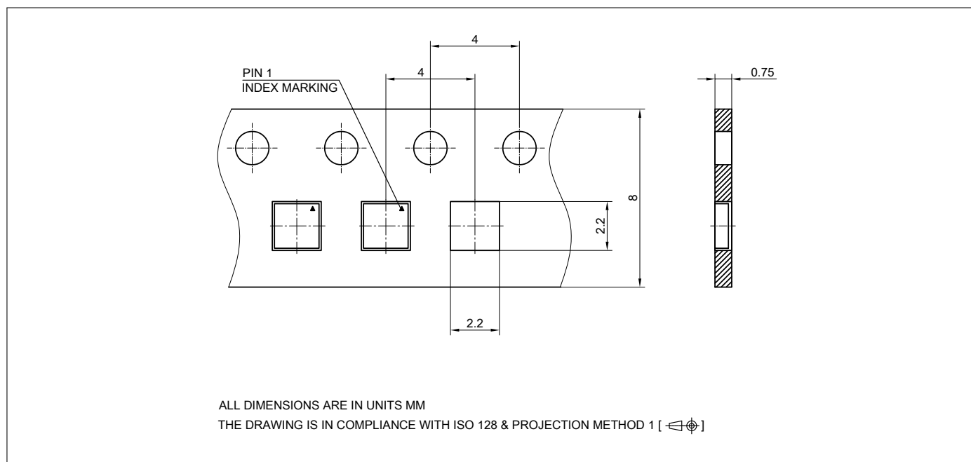
Figure 6: Carrier Tape
