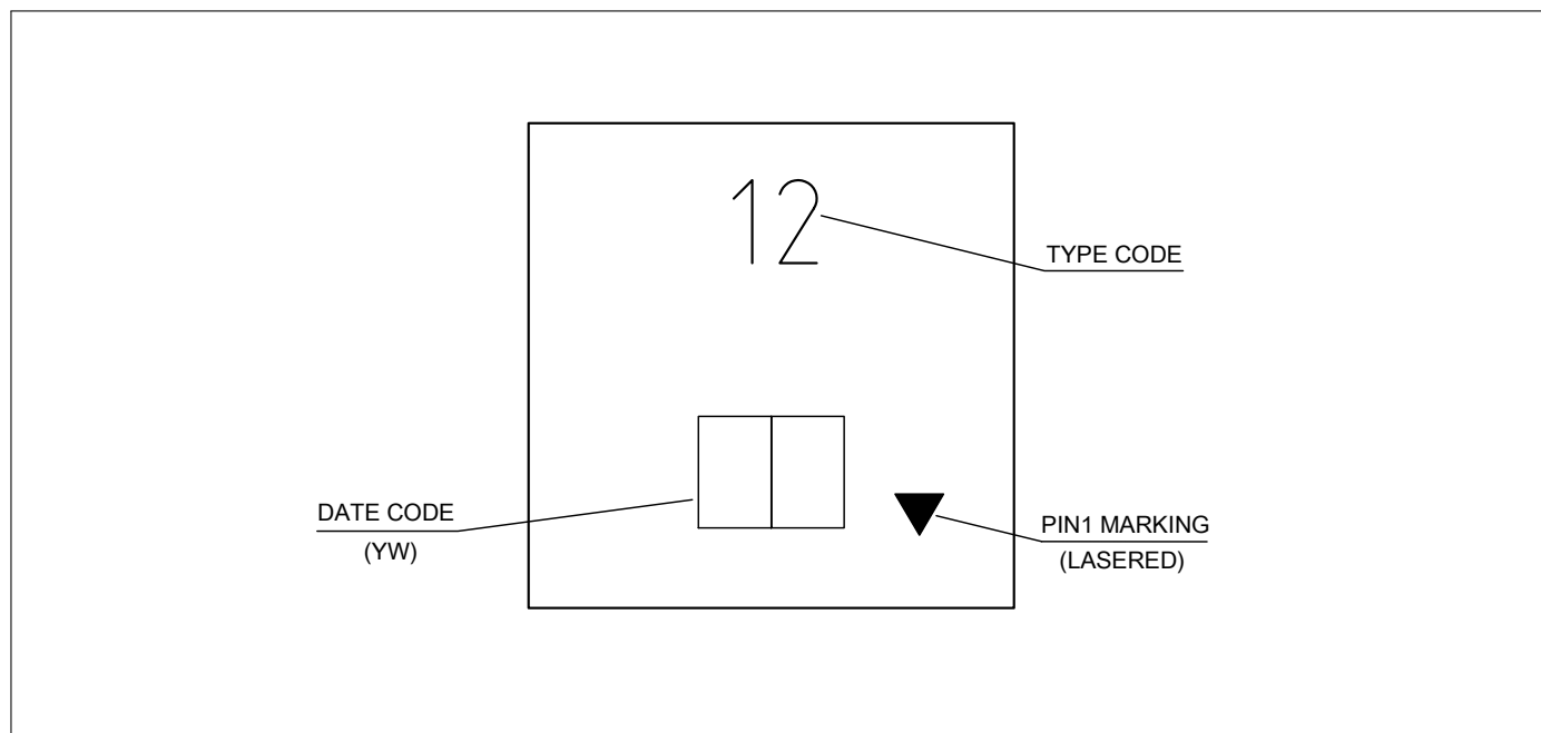
Figure 5: Laser marking
