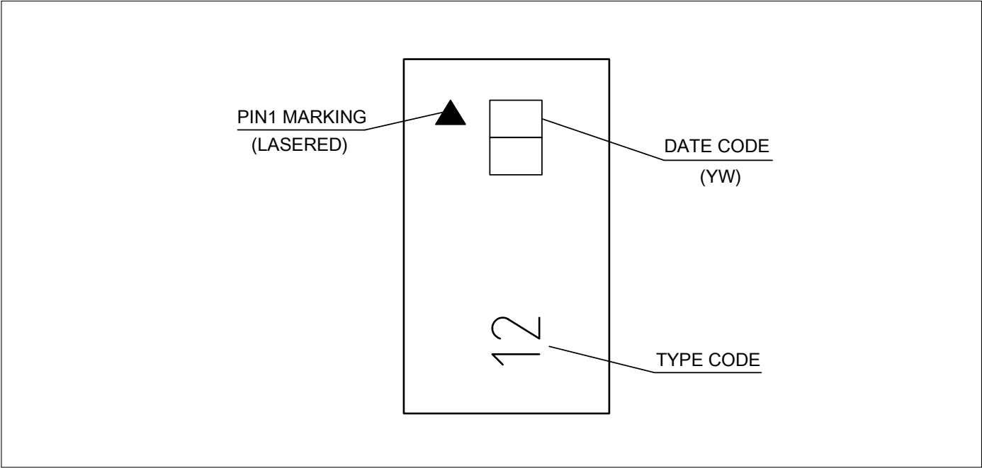
Figure 5: Laser marking
