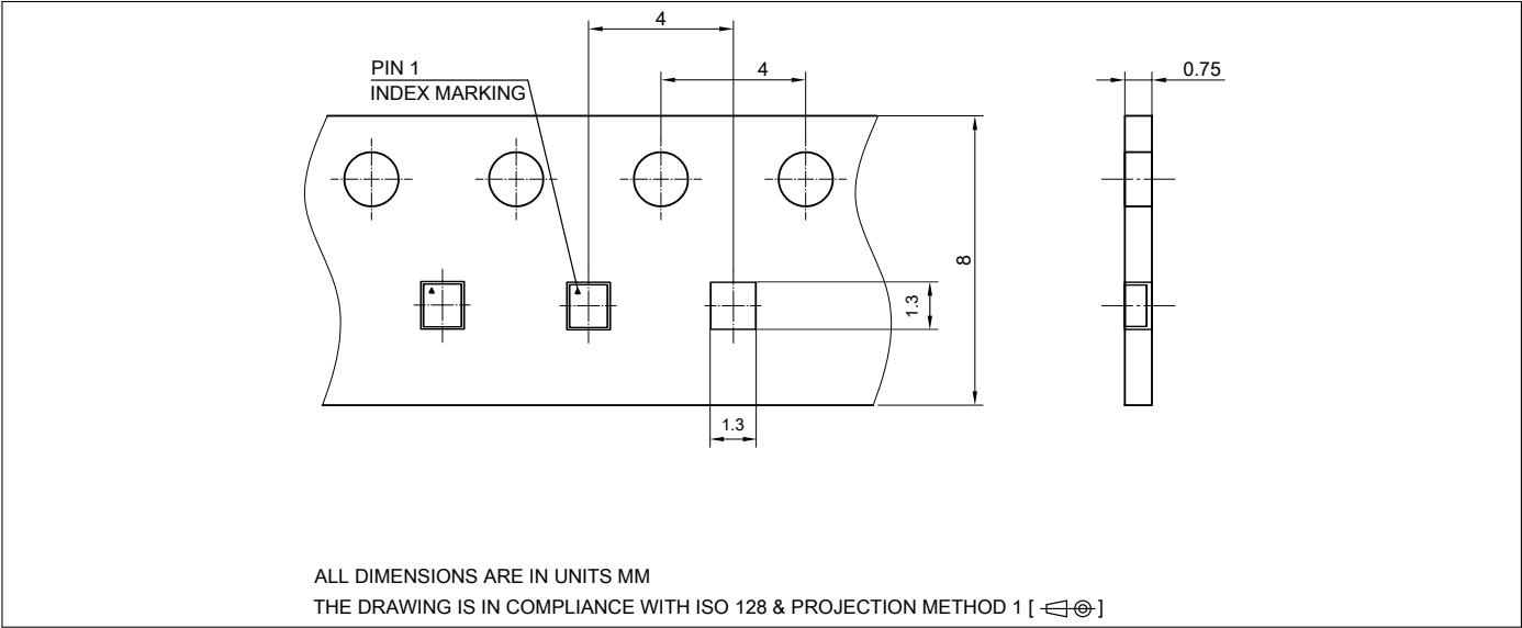
Figure 6: Carrier Tape
