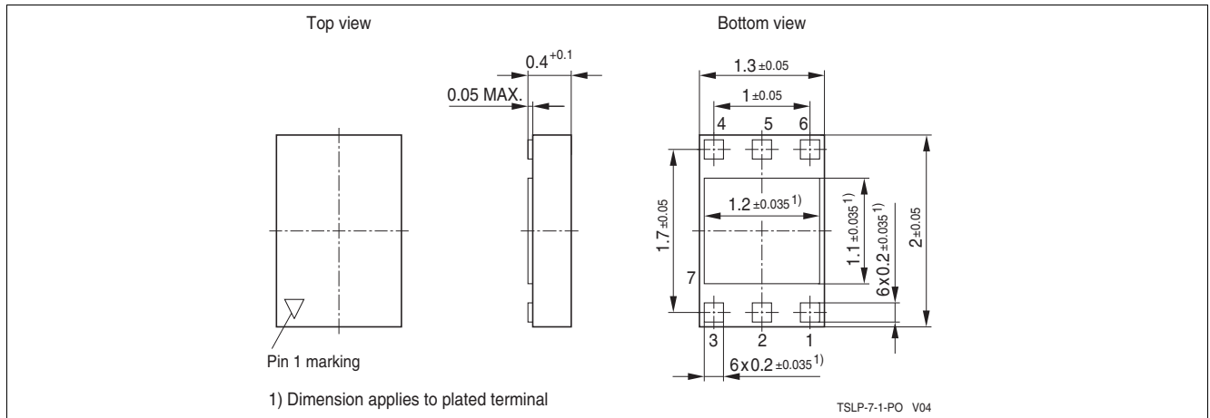
Figure 9-1 Package Outline of TSLP-7-1
