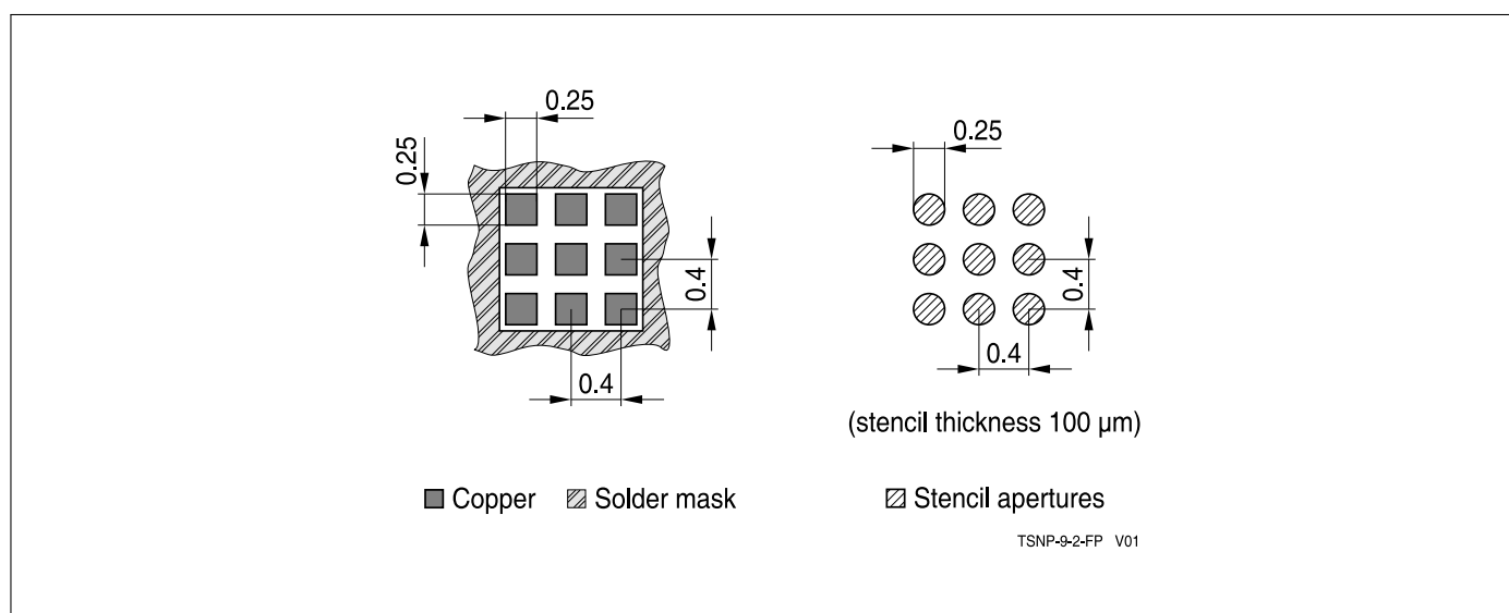
Figure 7: TSNP-9-2 Footprint Recommendation
