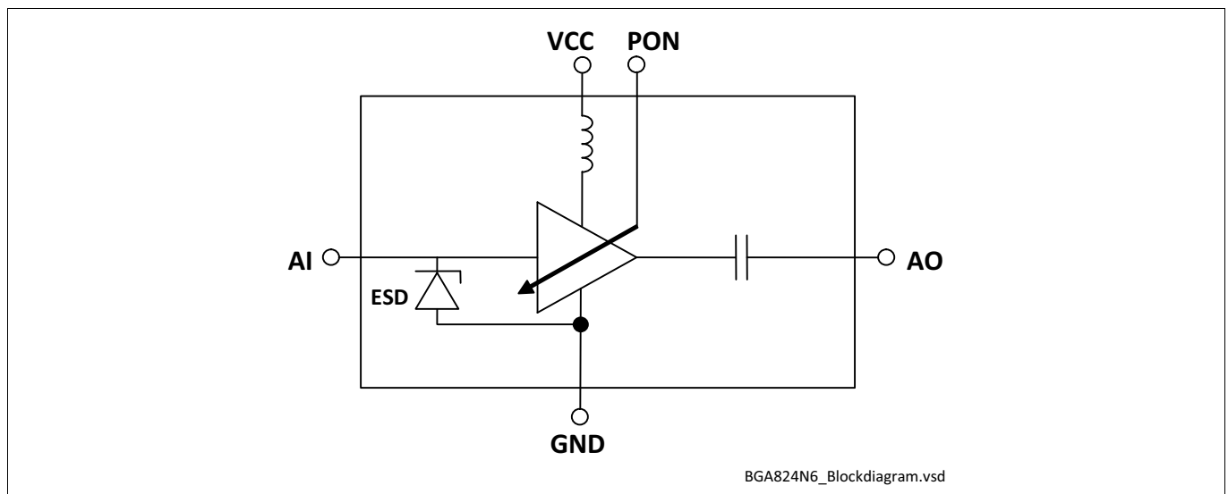
Figure 1 Block Diagram
