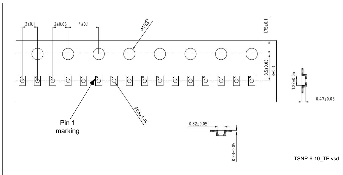
Figure 13 Tape &amp; Reel Dimensions TSNP-6-10 (reel diameter 180 mm, pieces/reel 12000)
