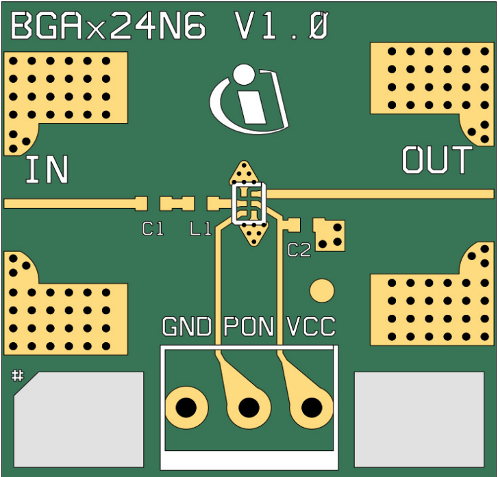
BGAx24N6_Application_Board.vsd
