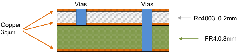
BGA824N6_application_board_sideview.vsd
