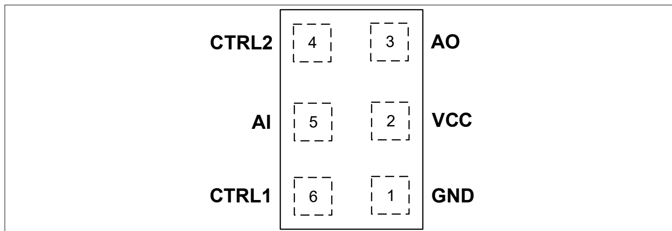
Figure 1: BGA535N6 pin configuration (top view)
